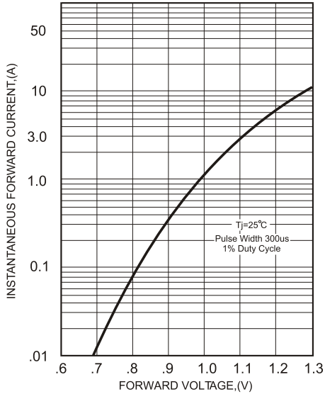
FIG.1-TYPICAL FORWARD CHARACTERISTICS
