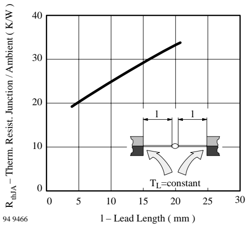
Figure 1. Max. Thermal Resistance vs. Lead Length
