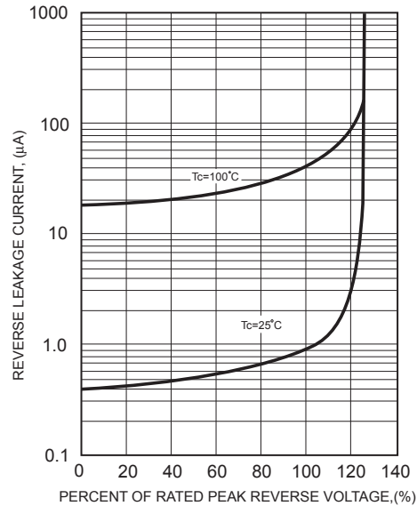
FIG.4-TYPICAL REVERSE CHARACTERISTICS
