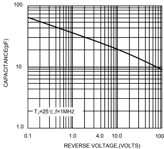
FIG.3-TYPICAL JUNCTION CAPACITANCE
