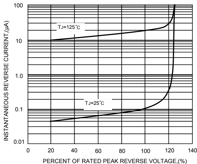
FIG.5-TYPICAL REVERSE CHARACTERISTICS
