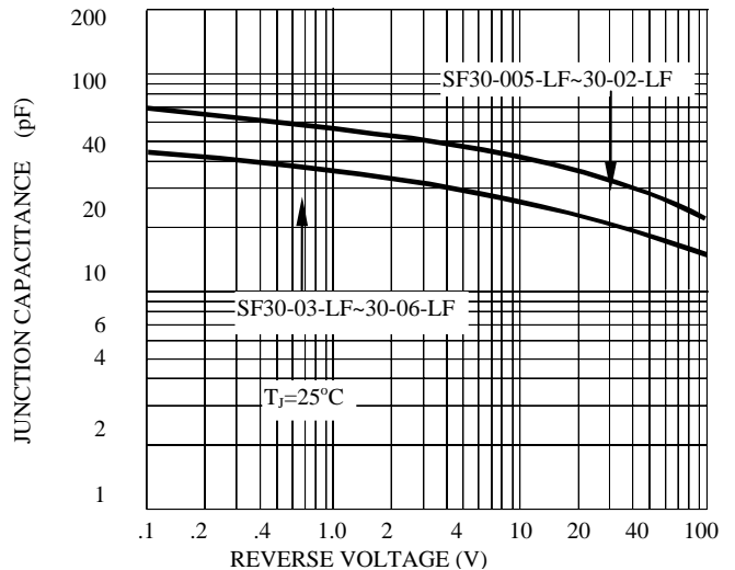
FIG. 6-TYPICAL JUNCTION CAPACITANCE
