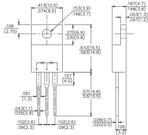
TO-220AB
