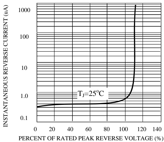
FIG. 3-TYPICAL REVERSE CHARACTERISTICS
