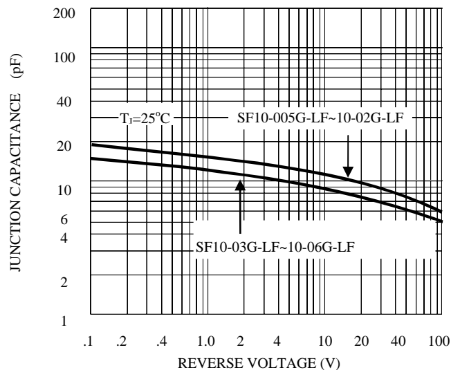
FIG. 6-TYPICAL JUNCTION CAPACITANCE
