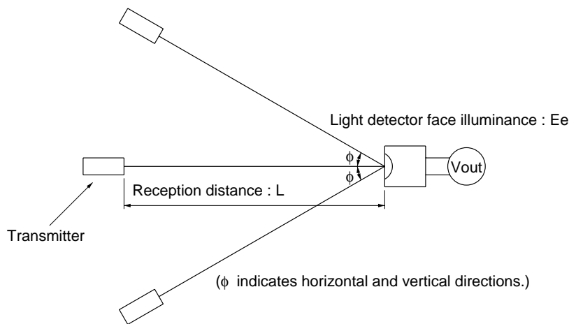
Fig. 2 Standard optical system
