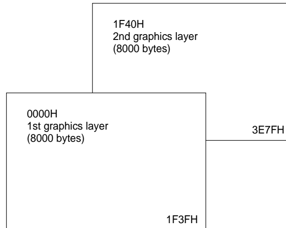
Figure 59. Two-layer graphics
