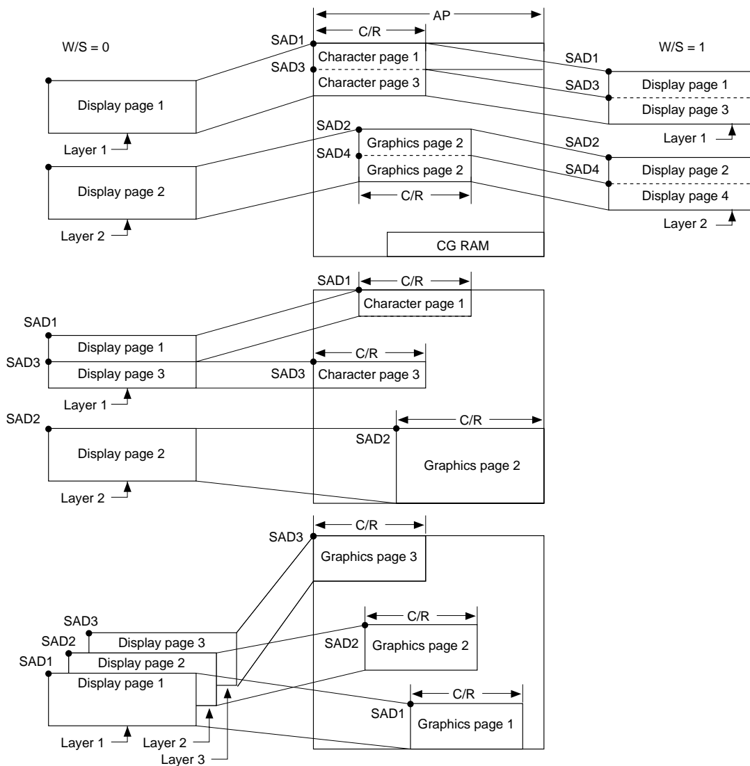
Figure 37. Display layers and memory
