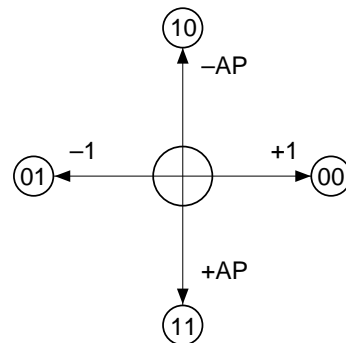
Figure 16. Cursor direction
