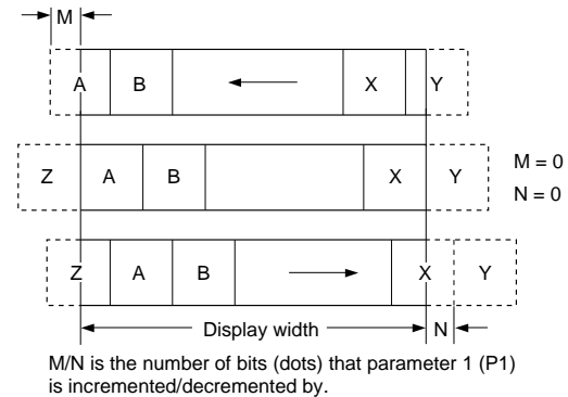
Figure 21. Horizontal scrolling
