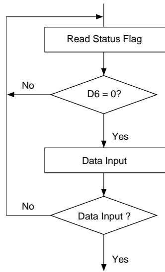
Figure 55. Flowchart for busy flag checking
