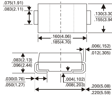
SMB/DO-214AA
