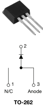
TO-262
