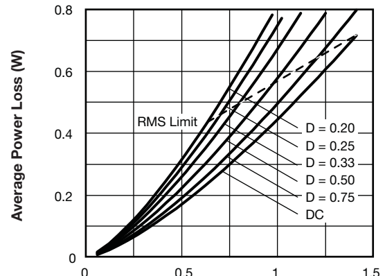
93256_05 Average Forward Current - I F(AV) (A) Fig. 5 - Forward Power Loss Characteristics
