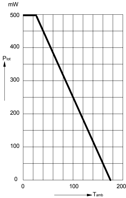
FIG.2 – ADMISSIBLE POWER DISSIPATION VERSUS AMBIENT TEMPERATURE
