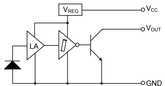
CLL135/CLL135W Open collector - inverter
