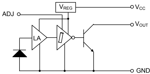
CLL133/CLL133W Open collector – inverter with Adjust
