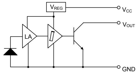
CLL134/CLL134W Open collector - buffer
