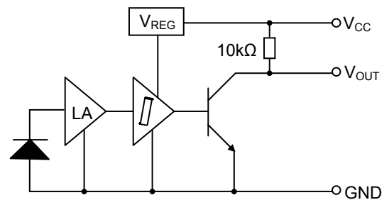
CLL136/CLL136W 10kΩ pull-up – buffer
