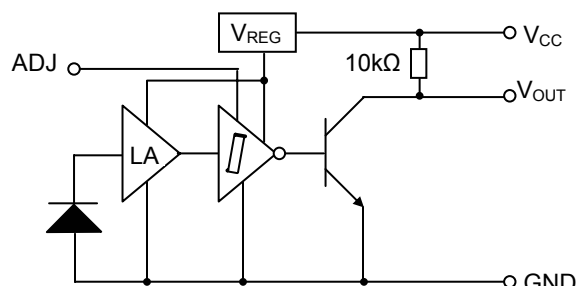
CLL131/CLL131W 10kΩ pull-up – inverter with Adjust
