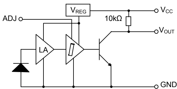
CLL130/CLL130W 10kΩ pull-up – buffer with Adjust
