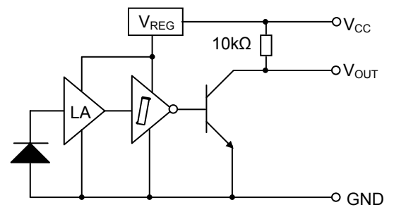
CLL137/CLL137W 10kΩ pull-up – inverter
