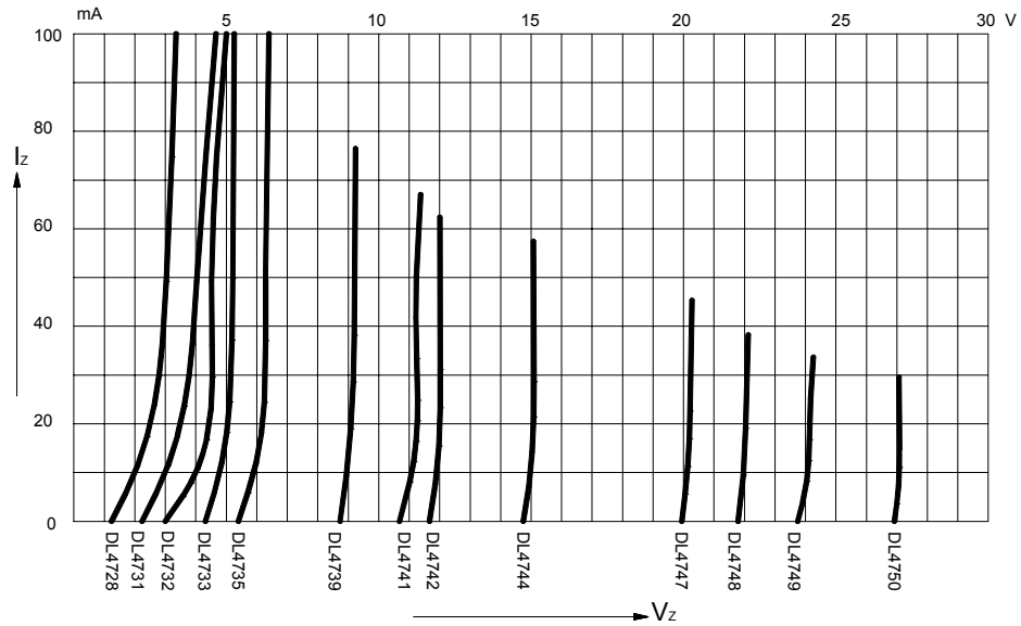
FIG.1 – BREAKDOWN CHARACTERISTICS
