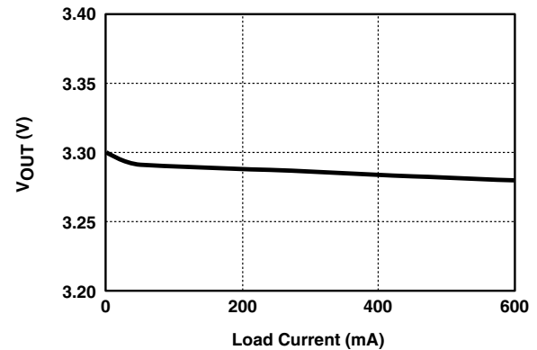
Figure 2. Load Regulation
