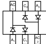
BAS70DW-04* Marking: K74
