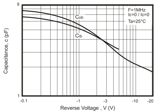
Fig. 6- C_{ob}/C_{ib} - V_{CB}/V_{EB}
