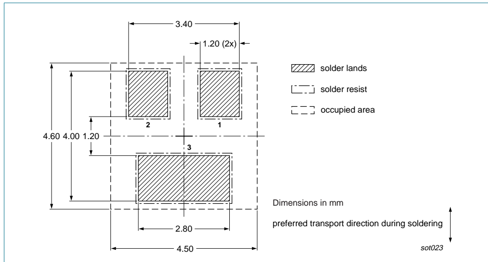
Fig 13. Wave soldering footprint BAW56 (SOT23/TO-236AB)
