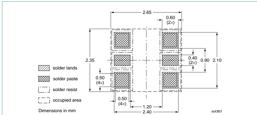
Fig 15. Reflow soldering footprint BAV756S and BAW56S (SOT363/SC-88)
