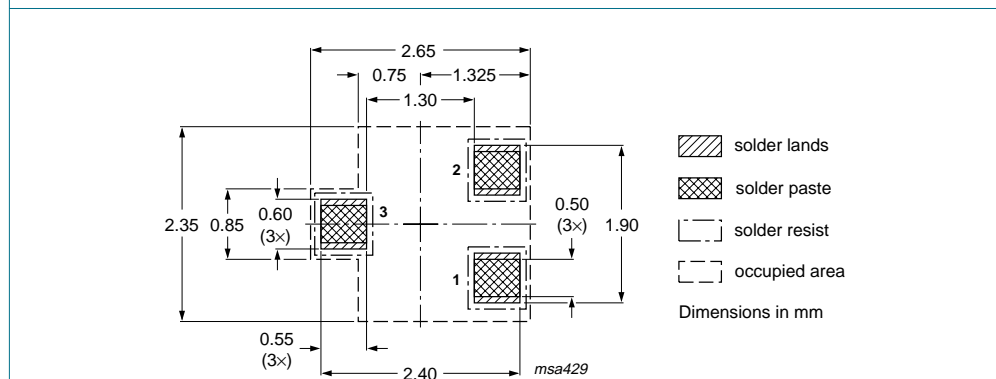
Fig 18. Reflow soldering footprint BAW56W (SOT323/SC-70)
