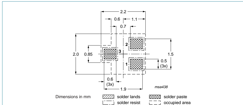
Fig 17. Reflow soldering footprint BAW56T (SOT416/SC-75)
