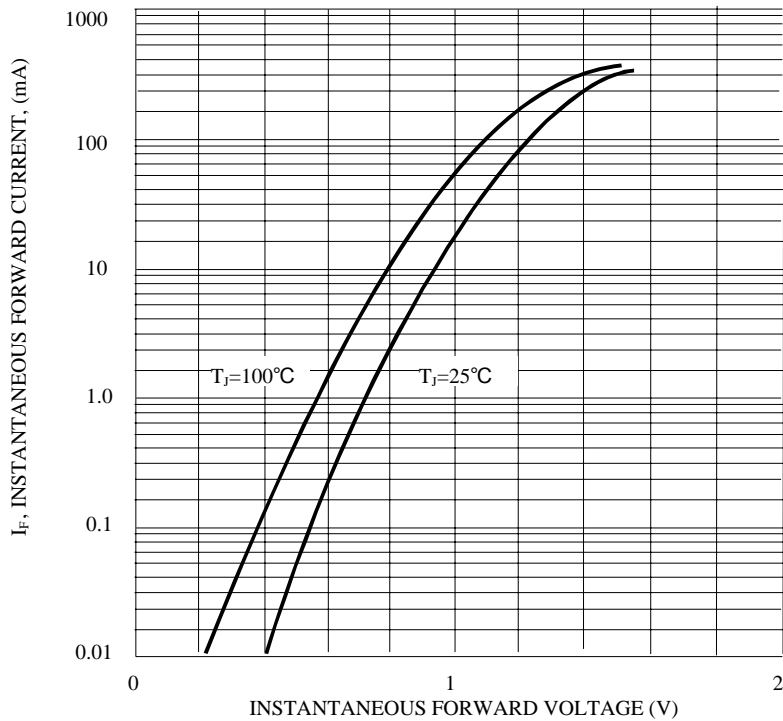
FIG.1 - FORWARD CHARACTERISTICS
