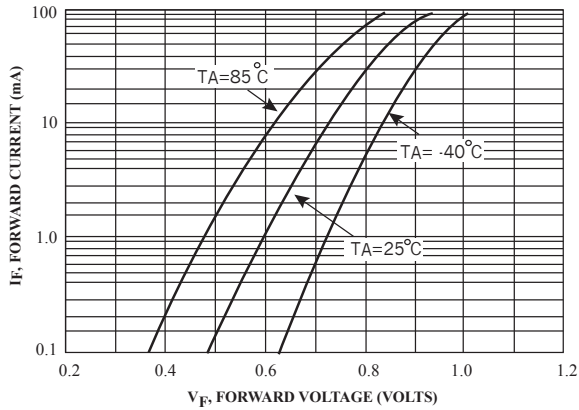
Figure 2. Forward Voltage
