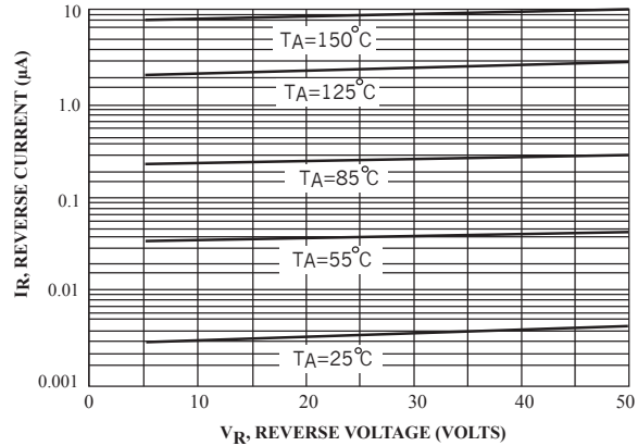
Figure 3. Leakage Current
