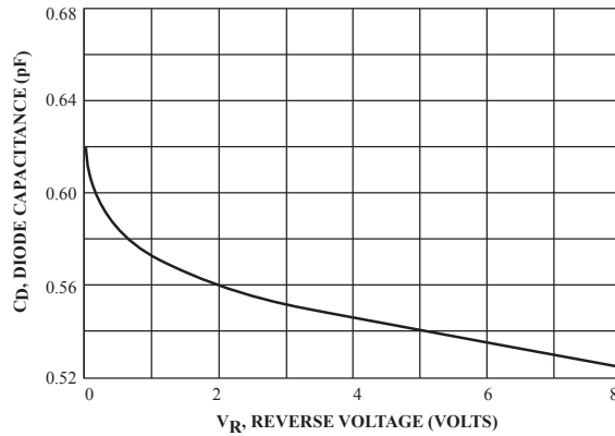
Figure 4. Capacitance
