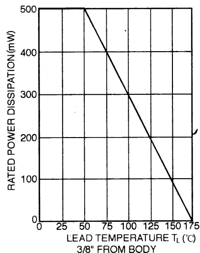
FIGURE 2 POWER DERATING CURVE
