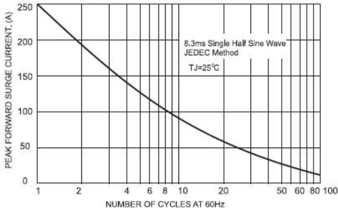
FIG.1- MAXIMUM NON-REPEITITIVE FORWARD SURGE CURRENT PER BRIDGE ELEMENT
