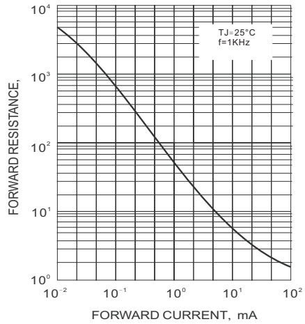
Fig.2-DYNAMIC FORWARD RESISTANCE VERSUS FORWARD CURRENT
