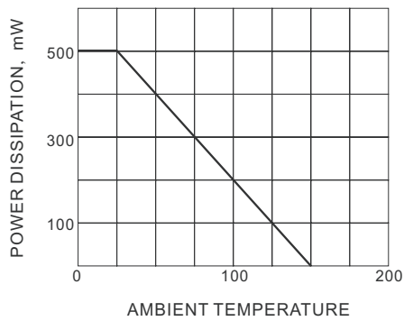
Fig.4 DERATING CURVE
