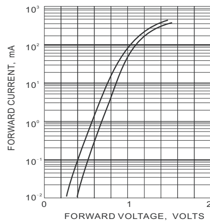
Fig.3 FORWARD CHARACTERISTICS
