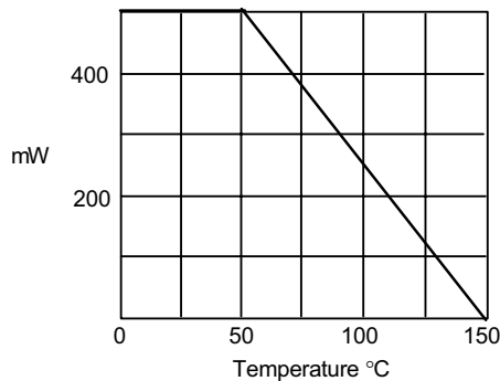
Power Dissipation (mW) - Versus - Temperature °C
