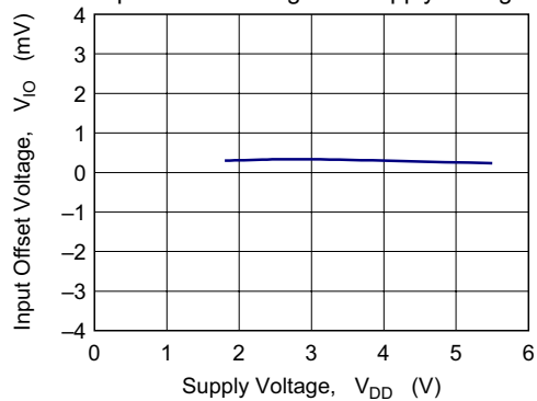
Figure 2-6 HA1631D02 Input Offset Voltage vs. Supply Voltage
