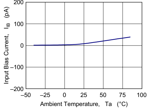
Figure 4-10 HA1631D04 Input Bias Current vs. Ambient Temperature
