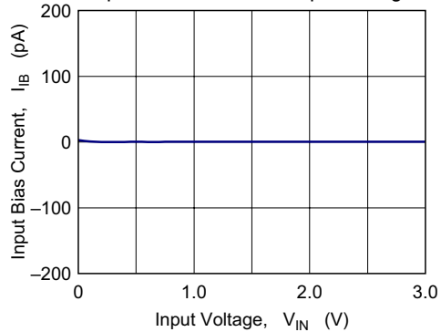
Figure 4-11 HA1631D04 Input Bias Current vs. Input Voltage
