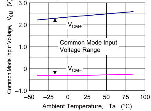
Figure 4-7 HA1631D04 Common Mode Input Voltage vs. Ambient Temperature
