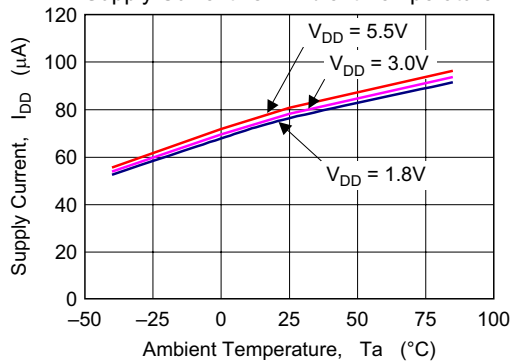
Figure 2-3 HA1631D02 Supply Current vs. Ambient Temperature
