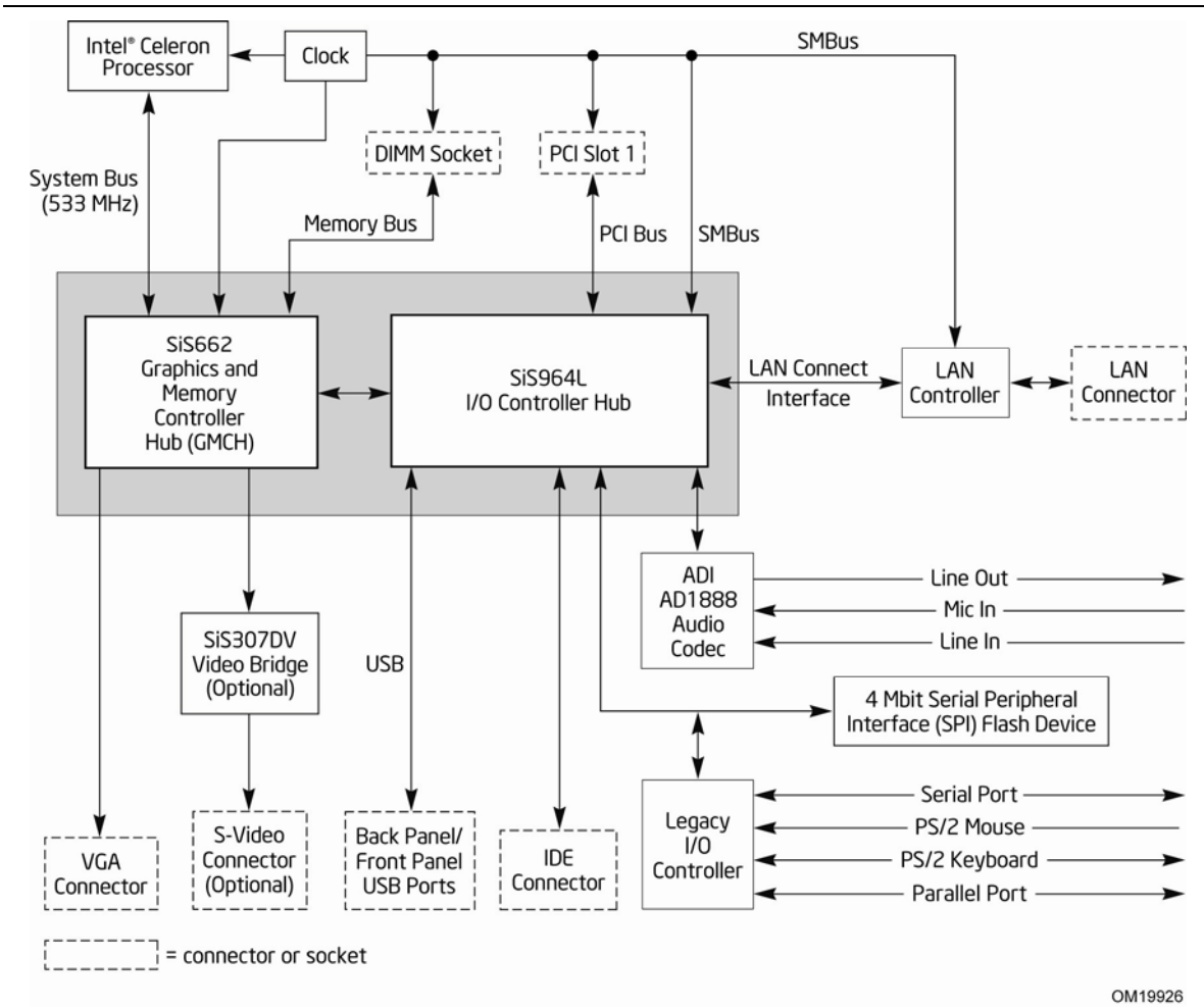
Figure 2. Block Diagram
