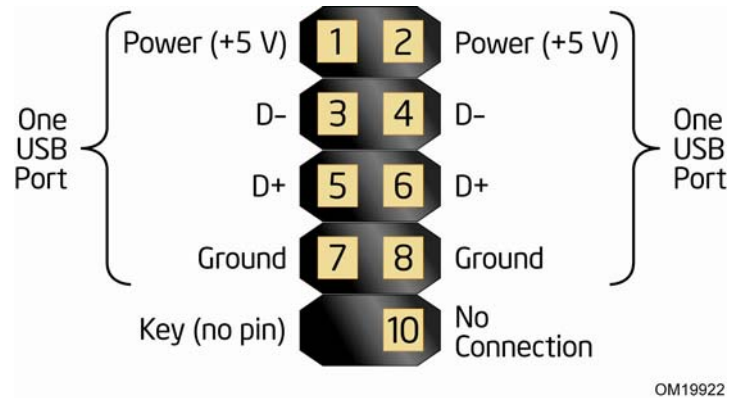
Figure 9. Connection Diagram for Front Panel USB Headers
