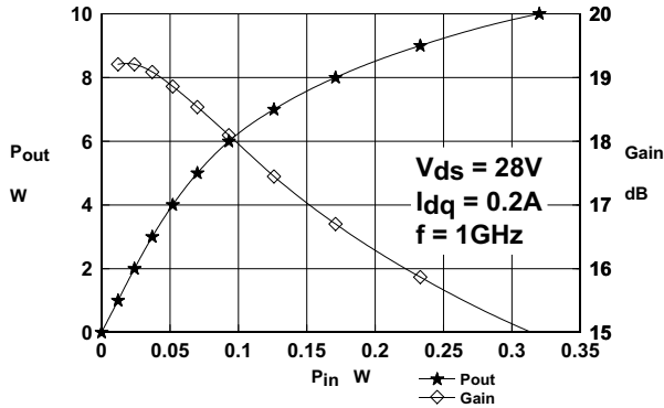
Figure 1 Output Power and Gain vs. Input power
