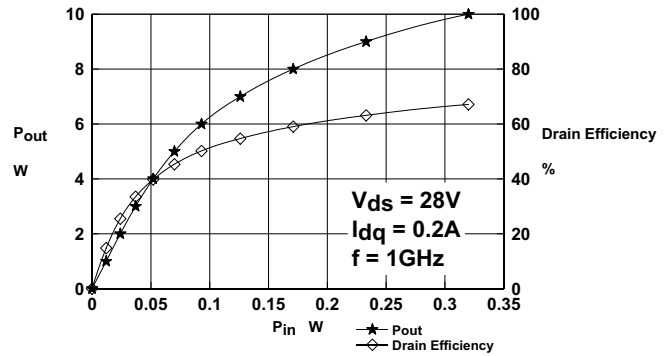
Figure 2 Output Power and Efficiency vs. Input Power
