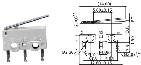
MP1_H01_ Lever Length = 14 mm
