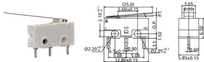
MP1_H02_ Lever Length = 25 mm
