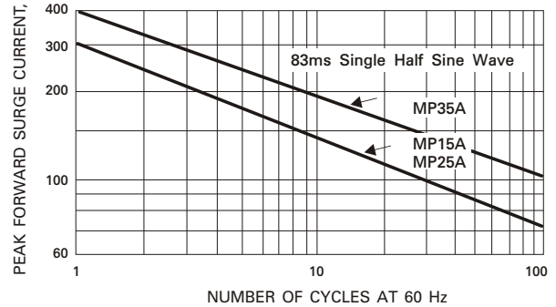
Fig. 2 - PAK FORWARD SURGE CURRENT
