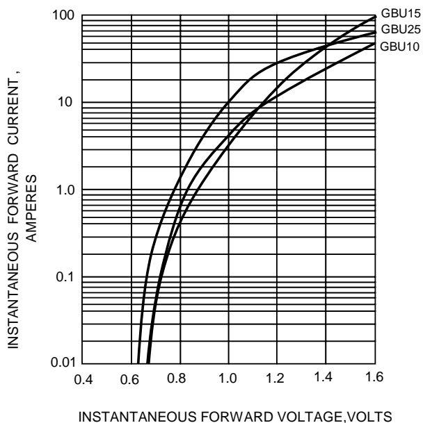
FIG.3-TYPICAL FORWARD CHARACTERISTICS
