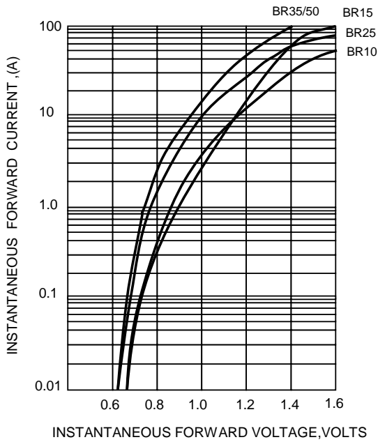
FIG.3-TYPICAL FORWARD CHARACTERISTICS
