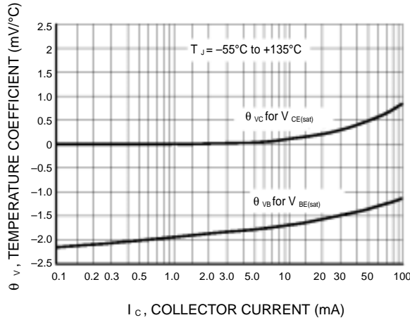
Figure 5. Temperature Coefficients
