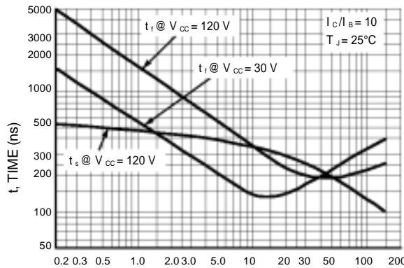
Figure 9. Turn-Off Time
