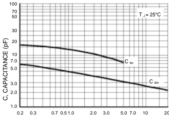
Figure 7. Capacitances Figure
