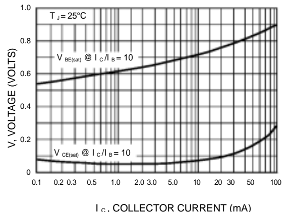
Figure 4. "On" Voltages
