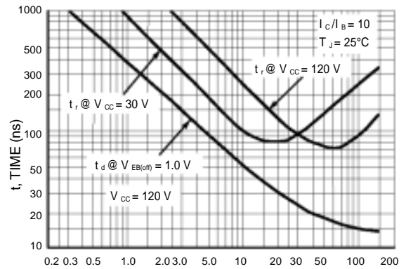
8. Turn-On Time
