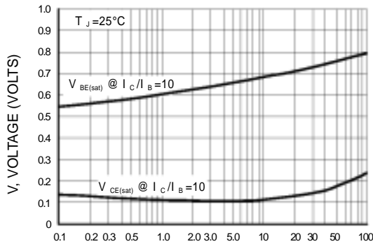
I_C , COLLECTOR CURRENT (mA) Figure 4. "On" Voltages
