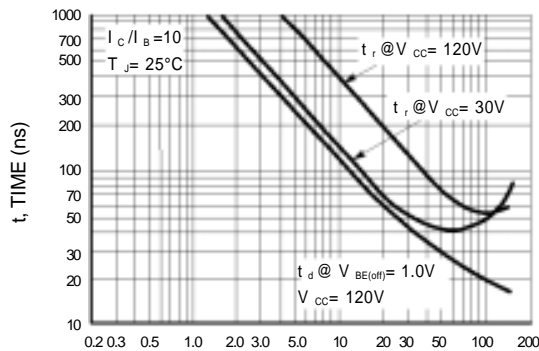
I_C , COLLECTOR CURRENT (mA) Figure 8. Turn-On Time
