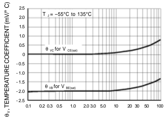
I_C , COLLECTOR CURRENT (mA) Figure 5. Temperature Coefficients
