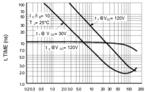
I_C , COLLECTOR CURRENT (mA) Figure 9. Turn-Off Time
