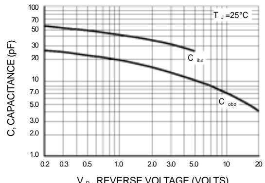
Figure 7. Capacitances
