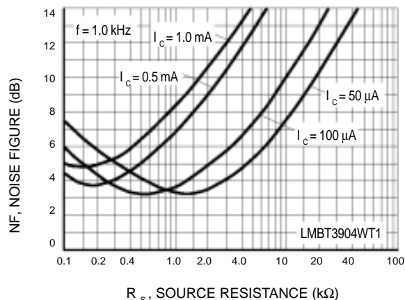
Figure 10. Noise Figure
