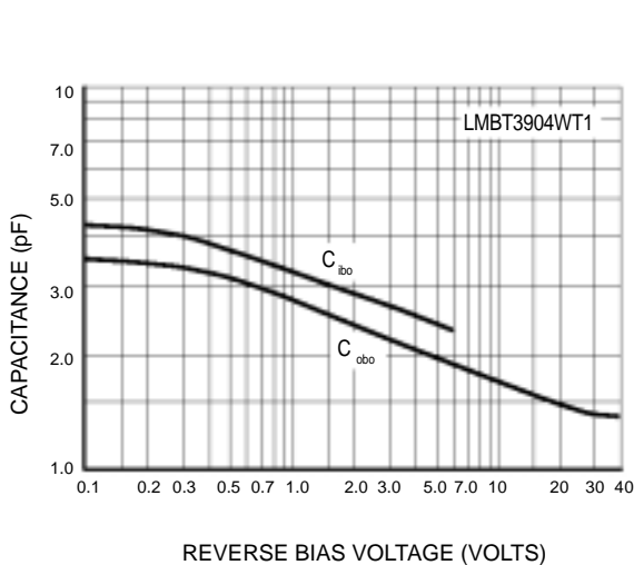
Figure 3. Capacitance
