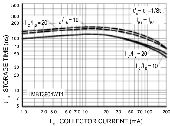
Figure 7. Storage Time
