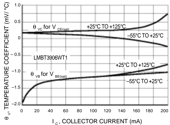
Figure 34. Temperature Coefficients
