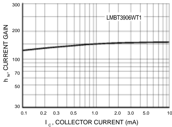
Figure 27. Current Gain
