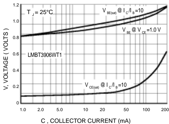
Figure 33. "ON" Voltages
