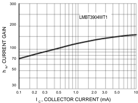
Figure 11. Current Gain
