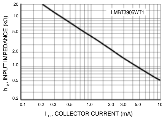
Figure 29. Input Impedance
