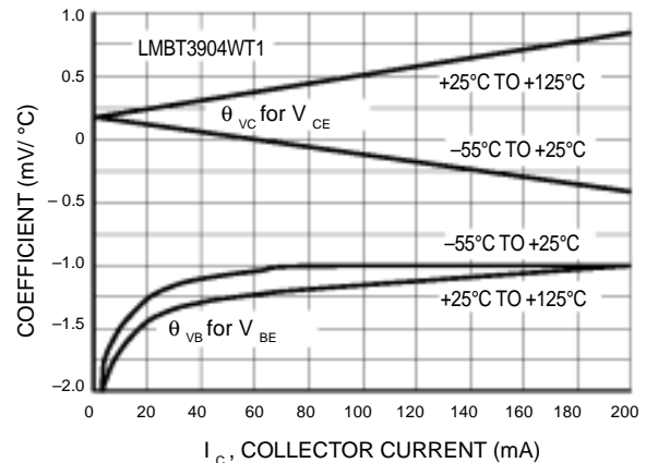
Figure 18. Temperature Coefficients
