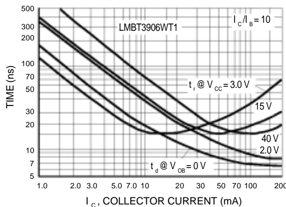
Figure 23. Turn-On Time
