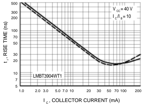
Figure 6. Rise Time
