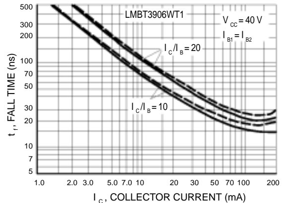
Figure 24. Fall Time
