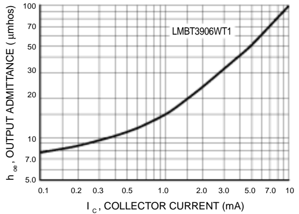
Figure 28. Output Admittance
