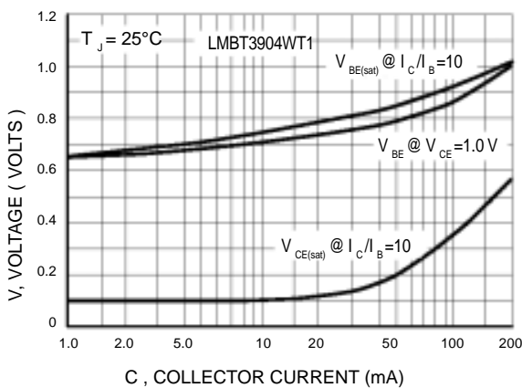
Figure 17. "ON" Voltages
