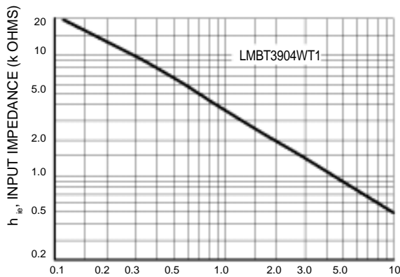
Figure 13. Input Impedance
