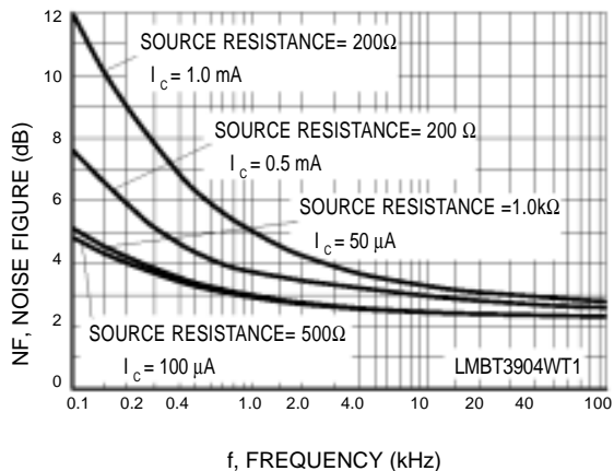
Figure 9. Noise Figure
