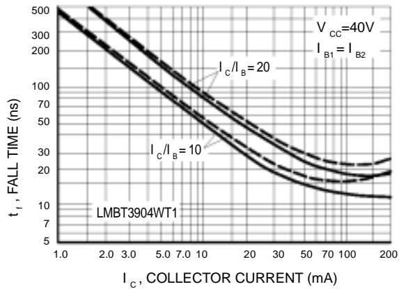
Figure 8. Fall Time
