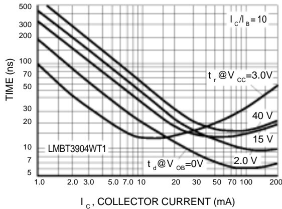
Figure 5. Turn-On Time
