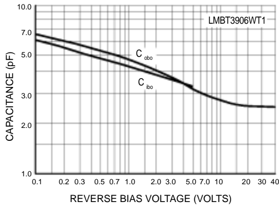
Figure 21. Capacitance
