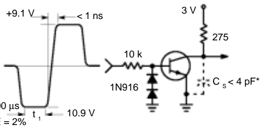
Figure 20. Storage and Fall Time Equivalent Test Circuit
