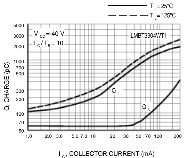
Figure 4. Charge Data
