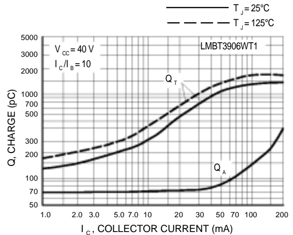
Figure 22. Charge Data
