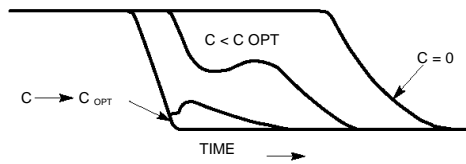
Figure 10. Turn-Off Waveform
