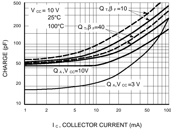
Figure 8. Maximum Charge Data
