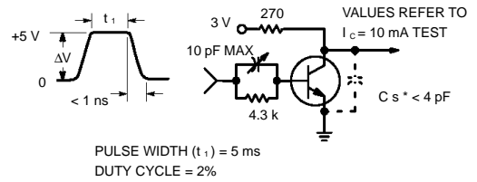
Figure 9. Q T Test Circuit
