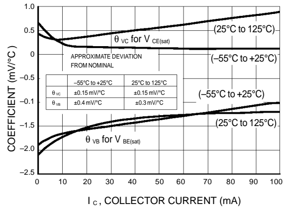
Figure 15. Typical Temperature Coefficients
