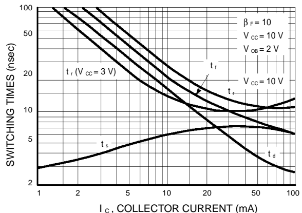
Figure 7. Typical Switching Times
