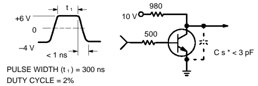
Figure 11. Storage Time Equivalent Test Circuit
