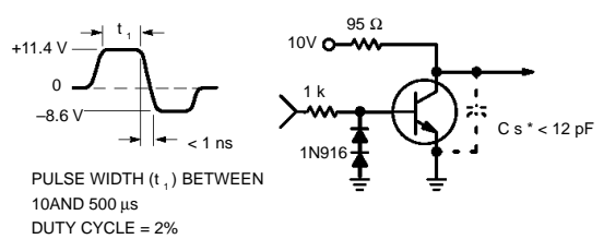
Figure 4. t_{off} Circuit — 100 mA
