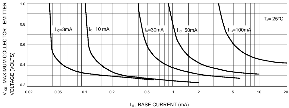
Figure 12. Maximum Collector Saturation Voltage Characteristics
