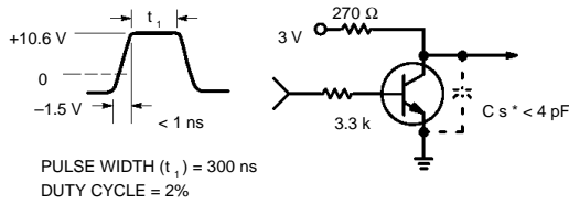
Figure 1. t_{on} Circuit — 10 mA
