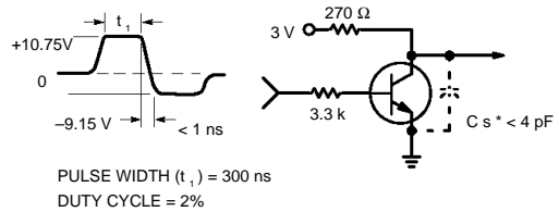
Figure 3. t_{off} Circuit — 10 mA
