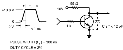
Figure 2. t_{on} Circuit — 100 mA
