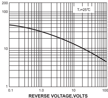
FIG. 5-TYPICAL JUNCTION CAPACITANCE
