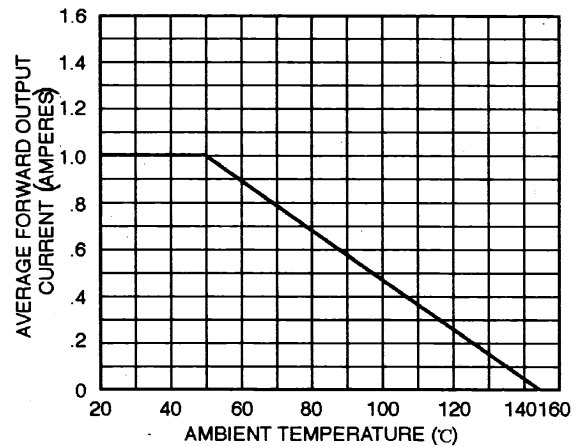
FIG.2 - TYPICAL FORWARD OUTPUT CURRENT DERATING CURVE
