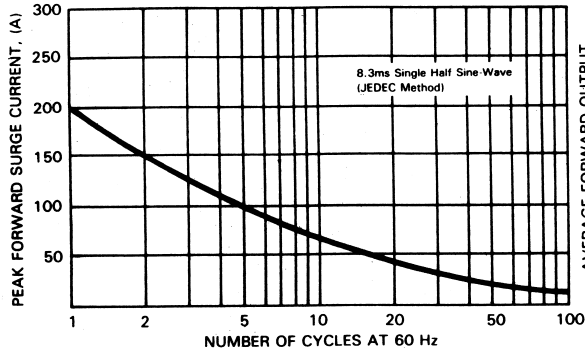
FIG.1-MAXIMUM NON-REPETITIVE FORWARD
