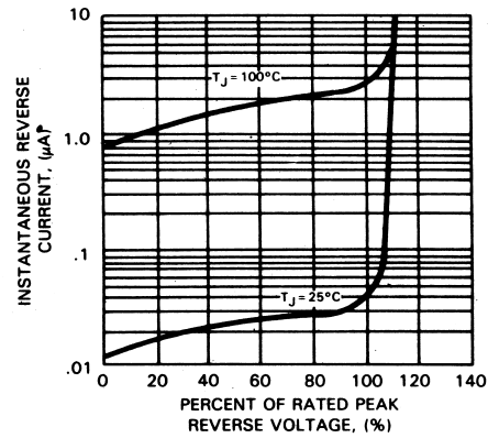
FIG.4-TYPICAL REVERSE CHARACTERISTICS
