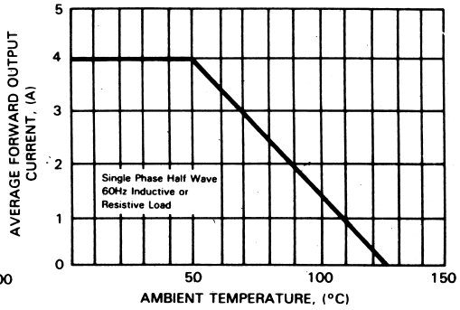
FIG.2-TYPICAL FORWARD CURRENT
