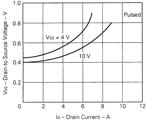
DRAIN TO SOURCE VOLTAGE vs. DRAIN CURRENT
