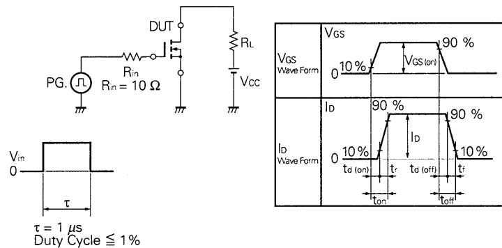
Fig. 1 Switching Test Circuit
