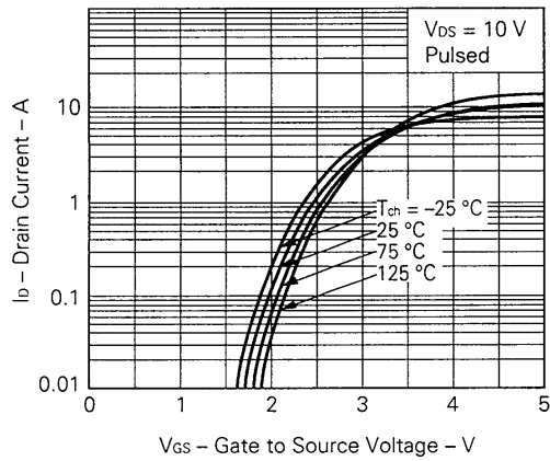
TRANSFER CHARACTERISTIC
