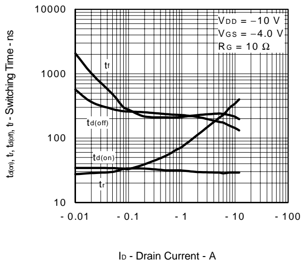
SWITCHING CHARACTERISTICS
