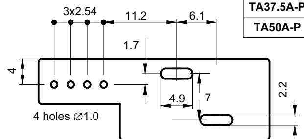
TA37.5A-P..TA50A-P PCB mounting hole layout
