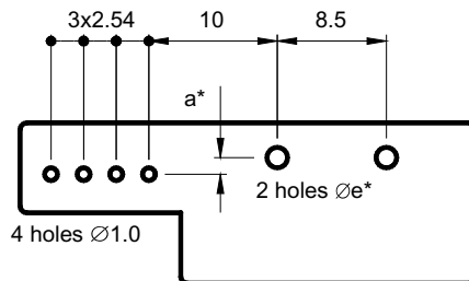
5A to 25A PCB mounting hole layout
