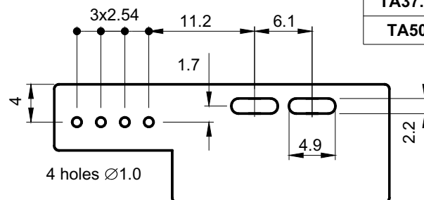
TA37.5A..TA50A PCB mounting hole layout
