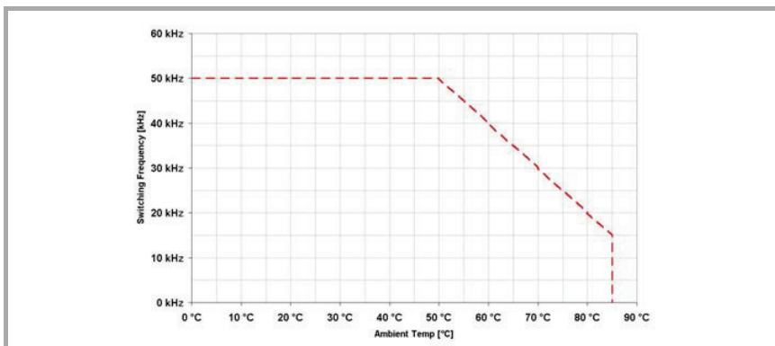
Derating
