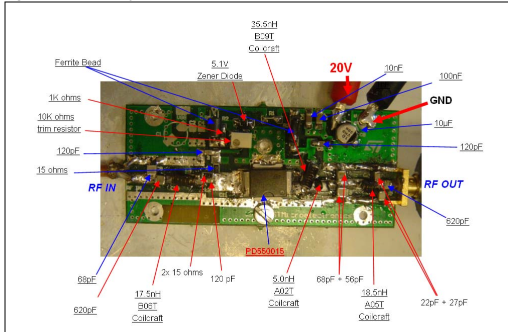
Figure 11. Circuit layout
