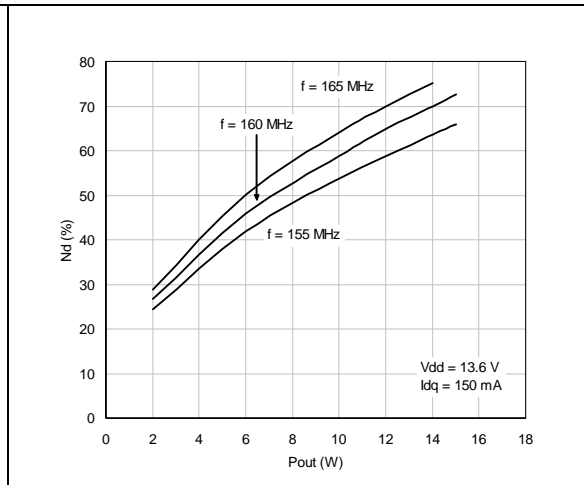
Figure 8. Efficiency vs P_{OUT} and frequency @ V_{DD} = 13.6 V
