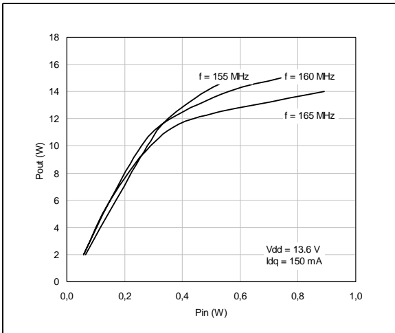
Figure 7. P_{OUT} vs pin and frequency @ V_{DD} = 13.6 V
