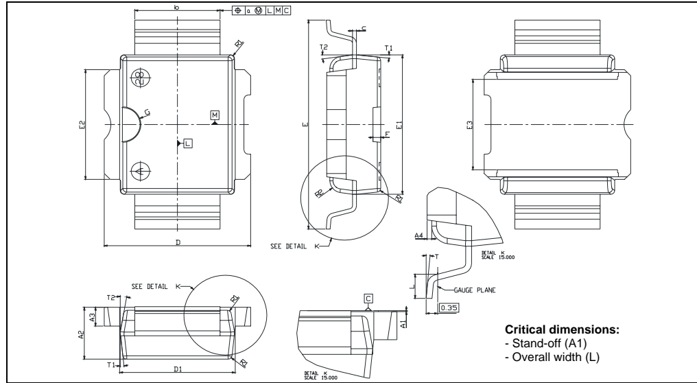
Figure 13. Package dimensions
