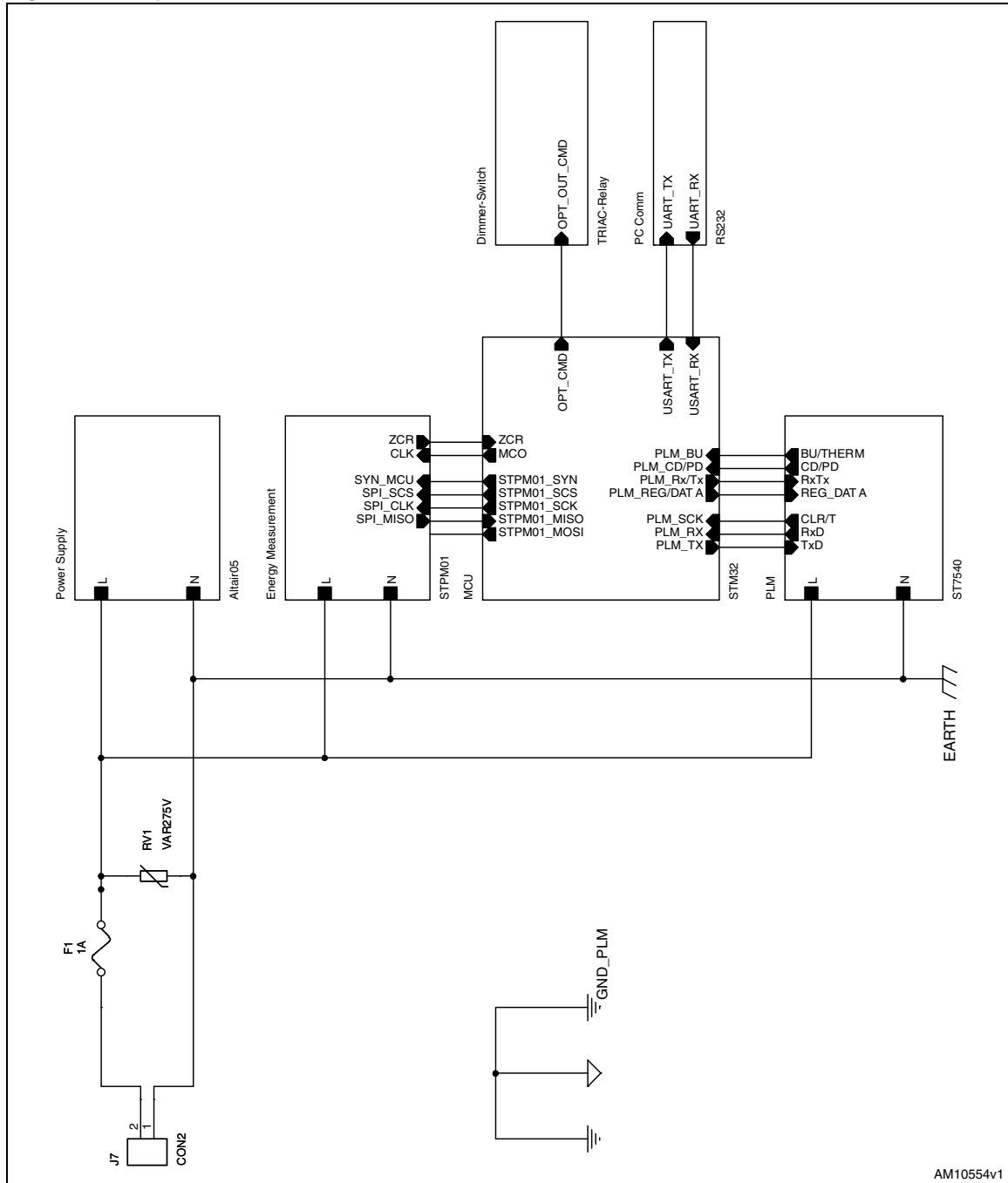
Figure 1. Top-level schematic
