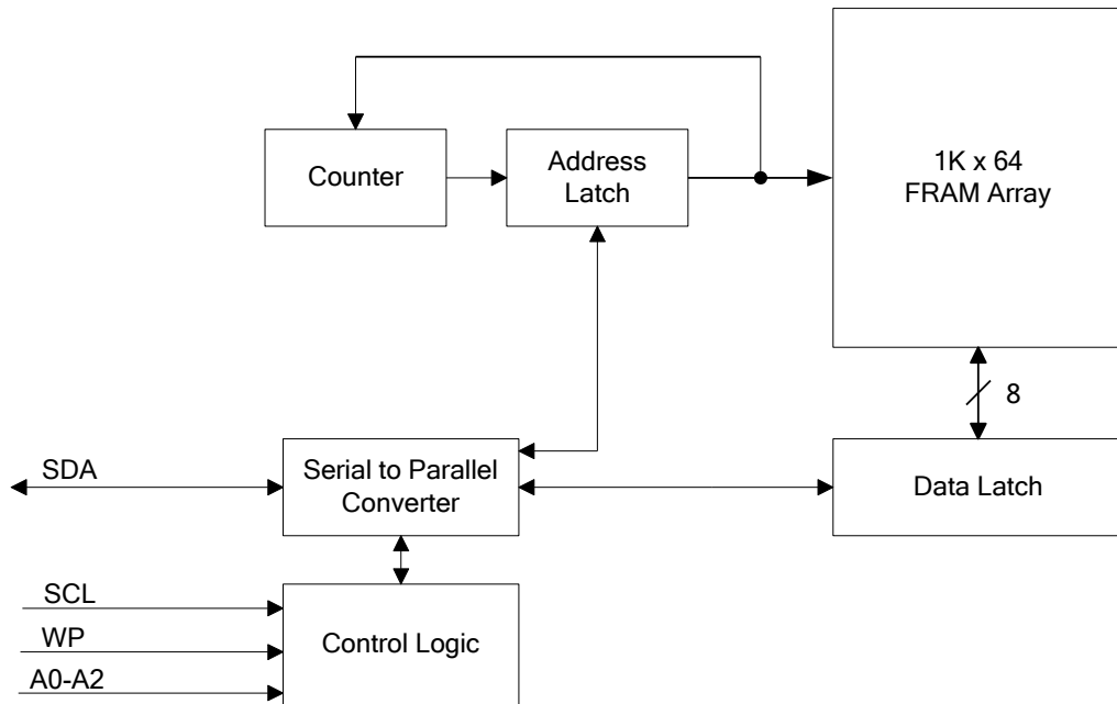
Figure 1. FM24CL64B Block Diagram
