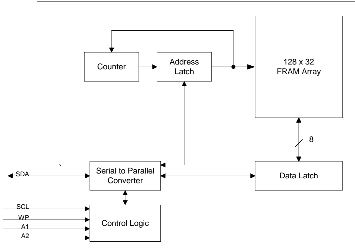
Figure 1. Block Diagram
