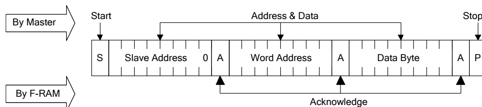
Figure 5. Byte Write
