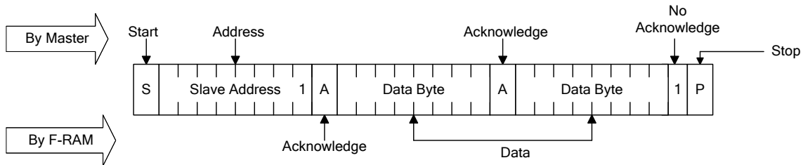
Figure 8. Sequential Read
