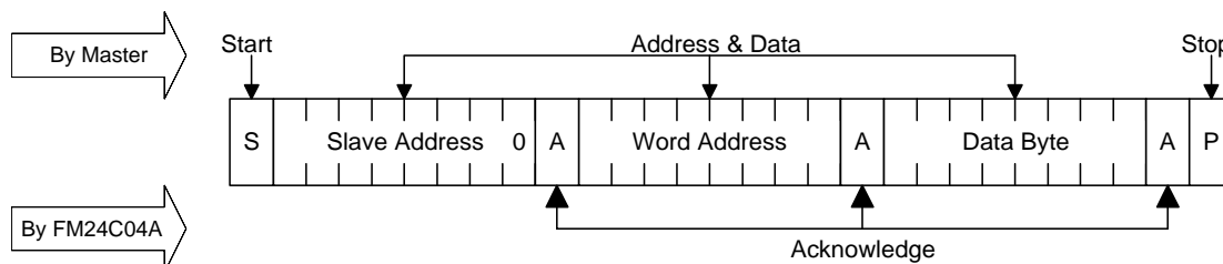
Figure 5. Byte Write
