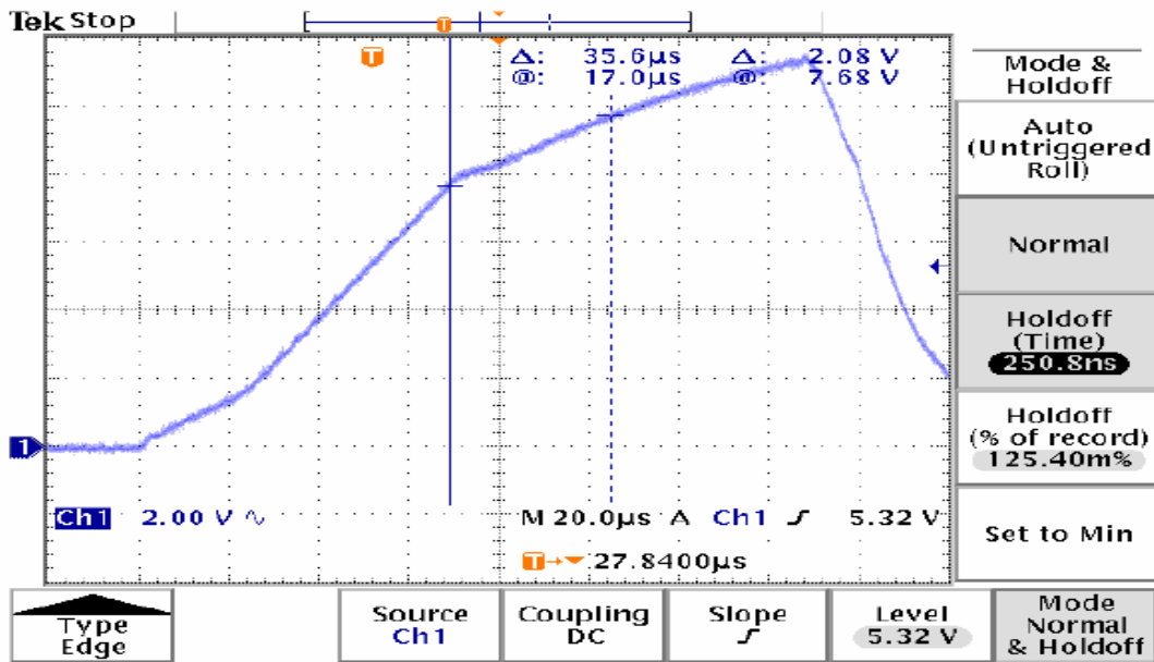
Clamping Voltage (Ipp = 7A , tp = 8/20 µs )
