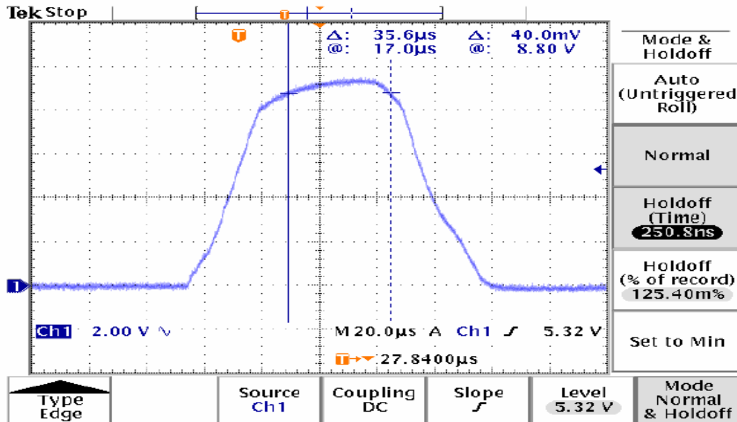
Clamping Voltage (Ipp = 1A , tp = 8/20 µs )
